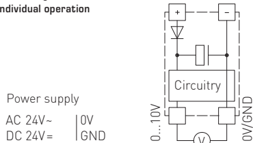
Connecting scheme Individual operation
